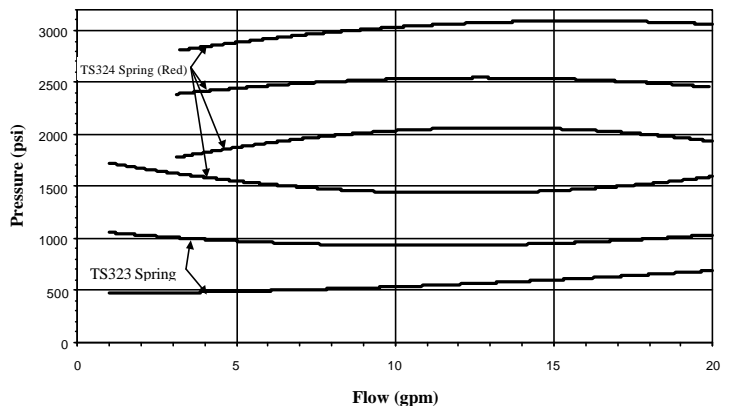
Pressure vs. Flow for RLC (0-20 gpm)
